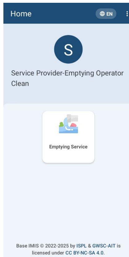
Figure 4-1 Dashboard
