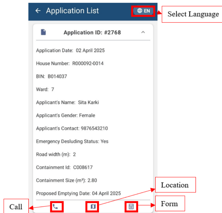
Figure 5-2 Application List
