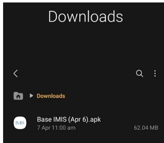
Figure 2-1 . APK file
